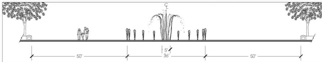
FOUNTAIN SECTION SCALE: 1/8" = 1'-0"
